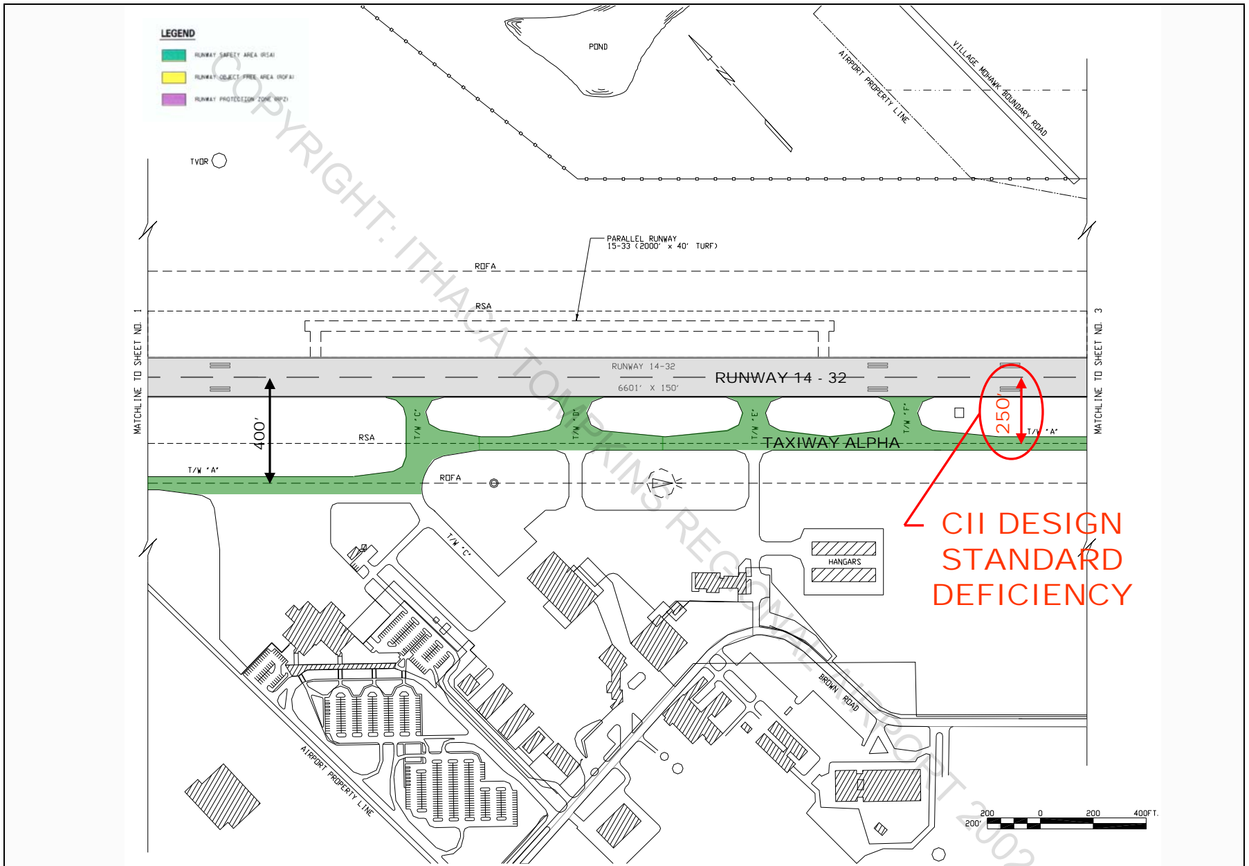
Ithaca Tompkins Regional Airport Runway 14-32 Extended Safety Area Analysis
