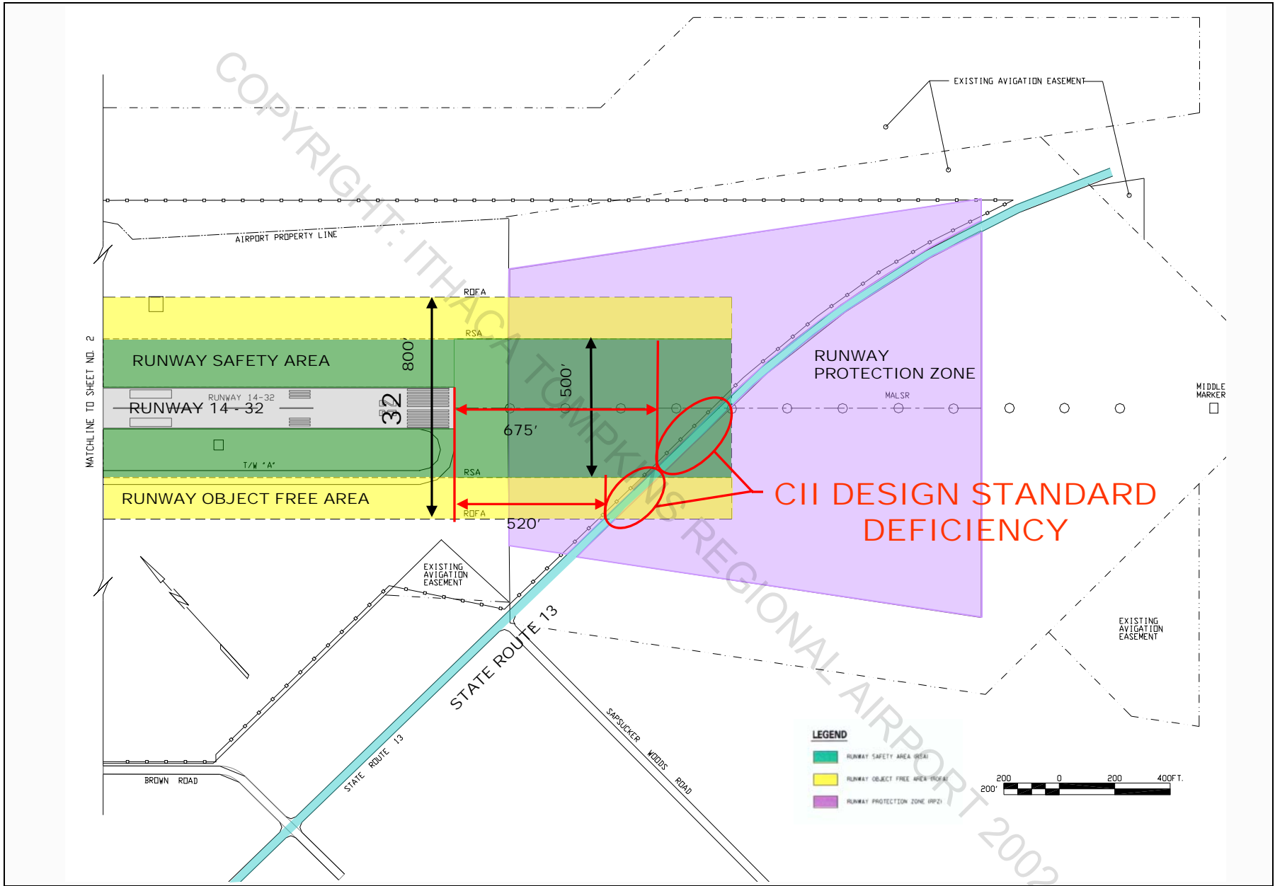
Approach Runway 32 Object Free Area & Safety Area Deficiency
